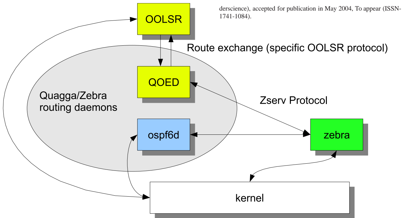
Fig. 5. Quagga OLSR interconnection architecture.
