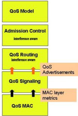
Fig. 2. The QoS support with its five components.
