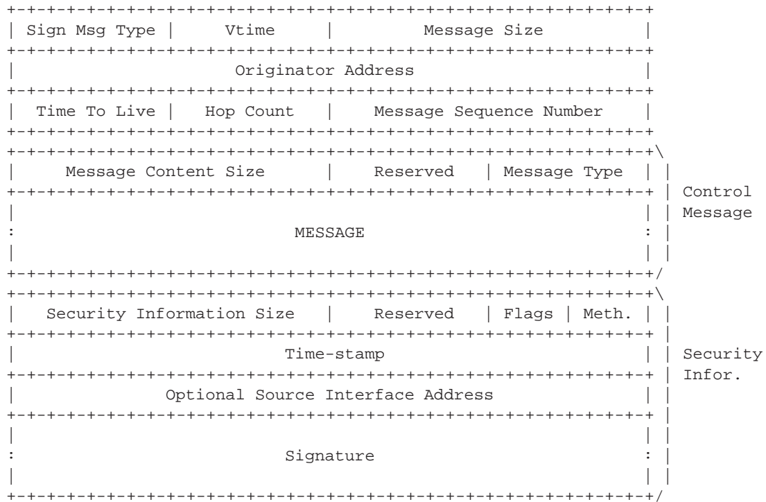
Fig. 3. Signed message format.
