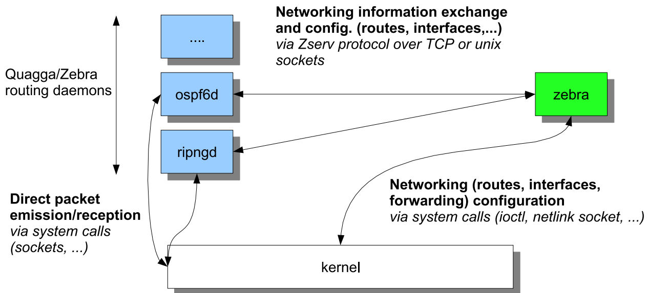
Fig. 4. Zebra/Quagga architecture.
