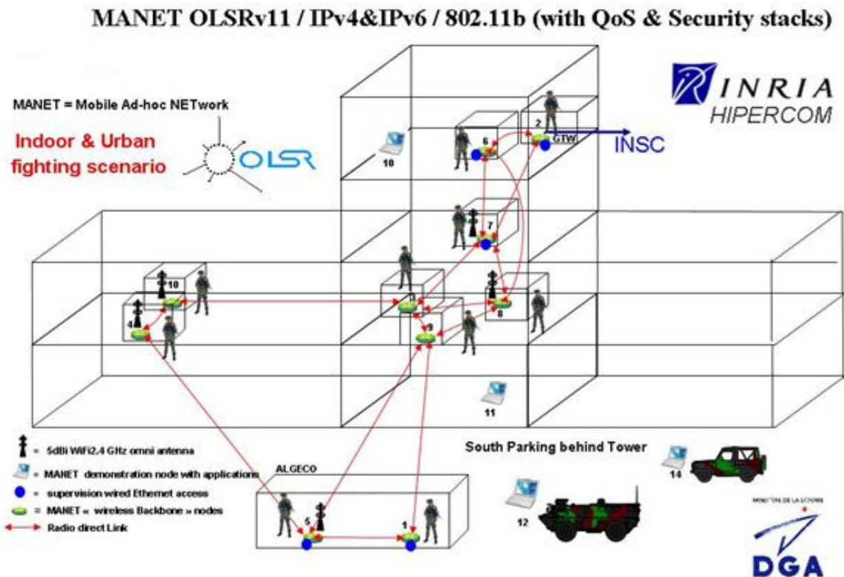
Fig. 1. The CELAR MANET/OLSR platform.
